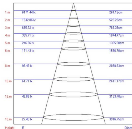
Lux-Distance Curve
